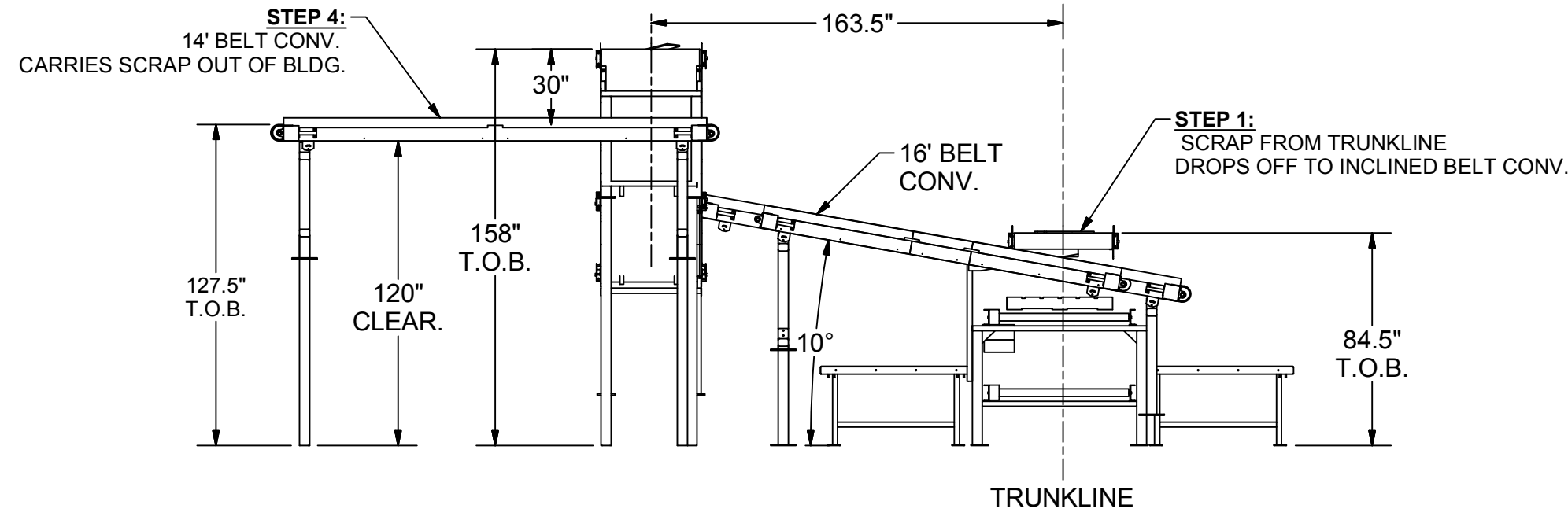
VIEW B-B
